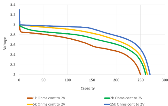
Continuous Discharge Characteristics
